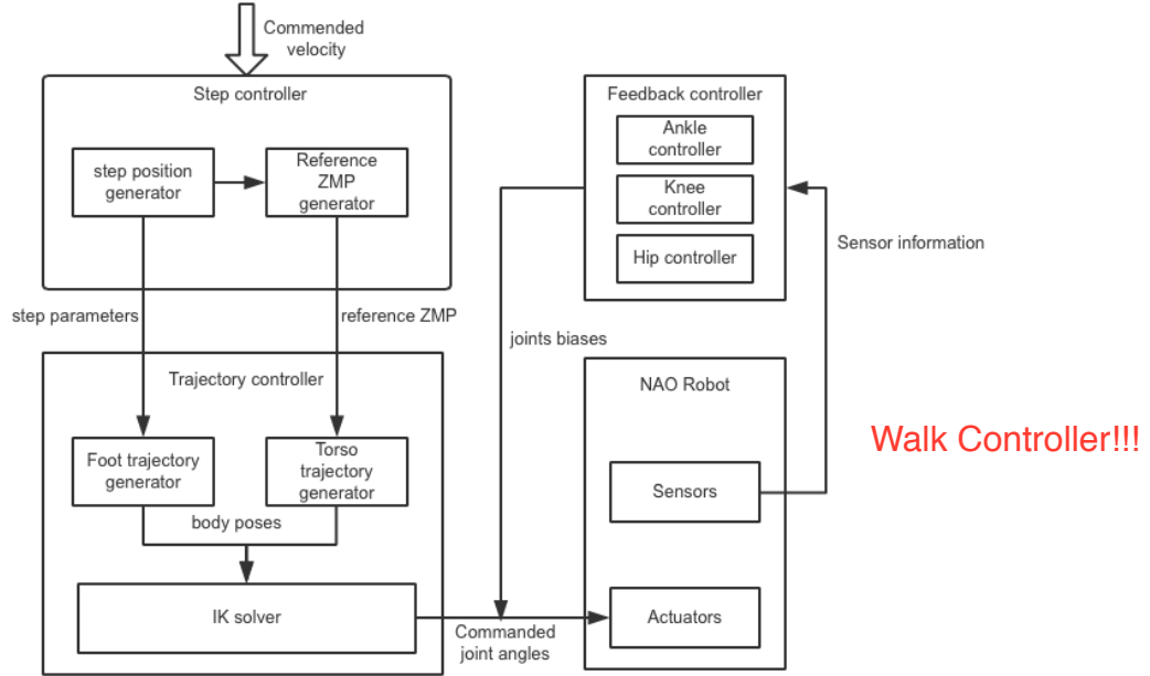
Fig. 2. Overview of the walk controller
