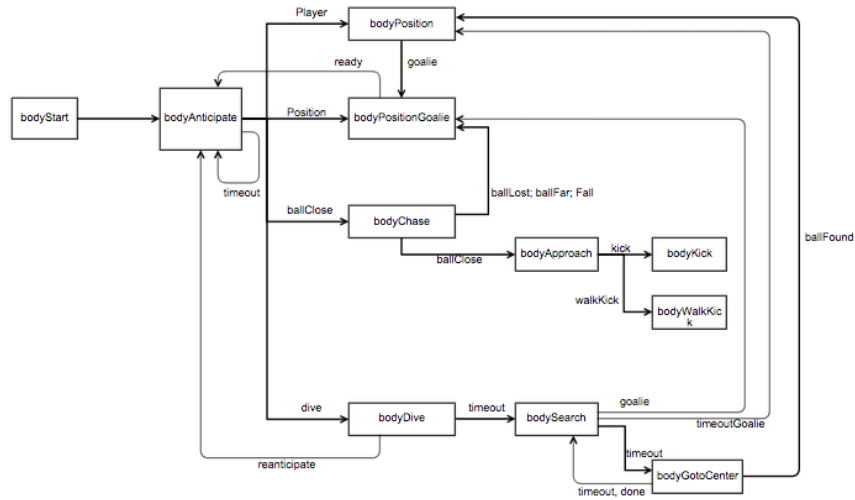
Fig. 17. Body State Machine for a goalie.
